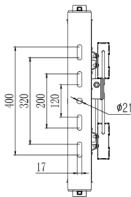
Dimensional Drawing of Bracket.
